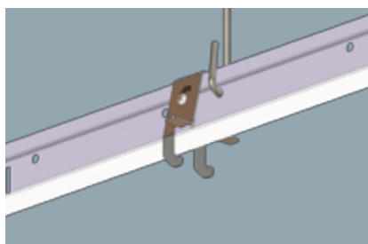
Montage Cross-Lock verbinding
